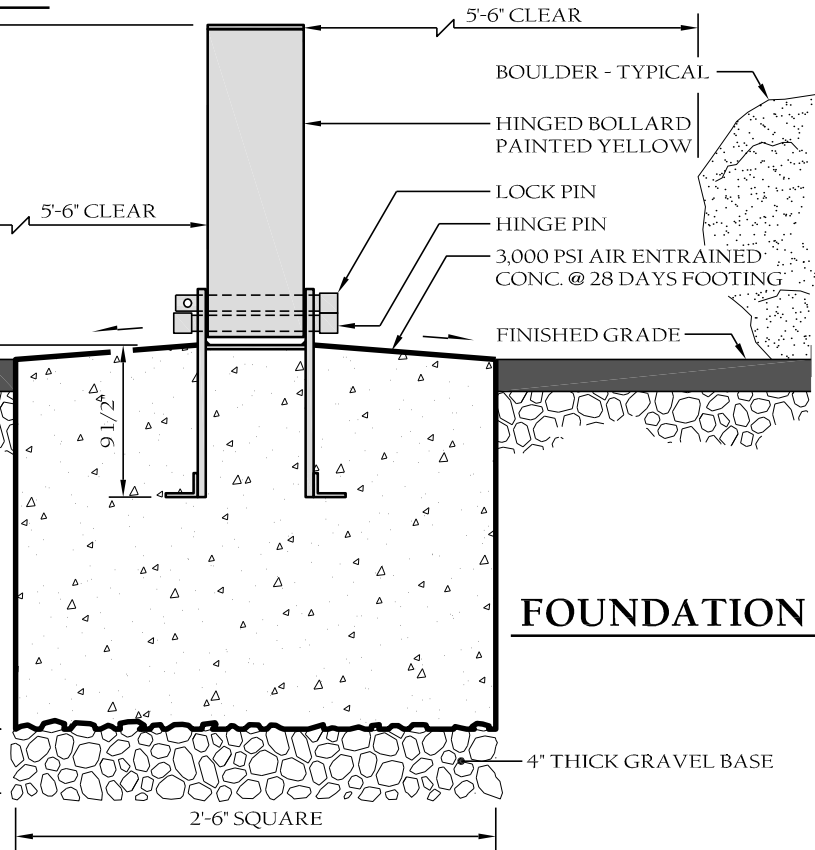
HINGED BOLLARD DETAIL
